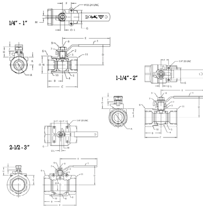
STAINLESS STEEL BALL VALVE
