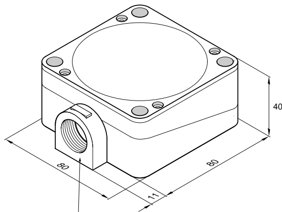
(1/2"-14 NPT) Internal Thread with Screw Terminals
